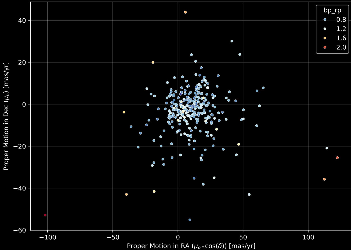
GALAH DR4 Field: [6965] Proper Motion Diagram (n= 306)
