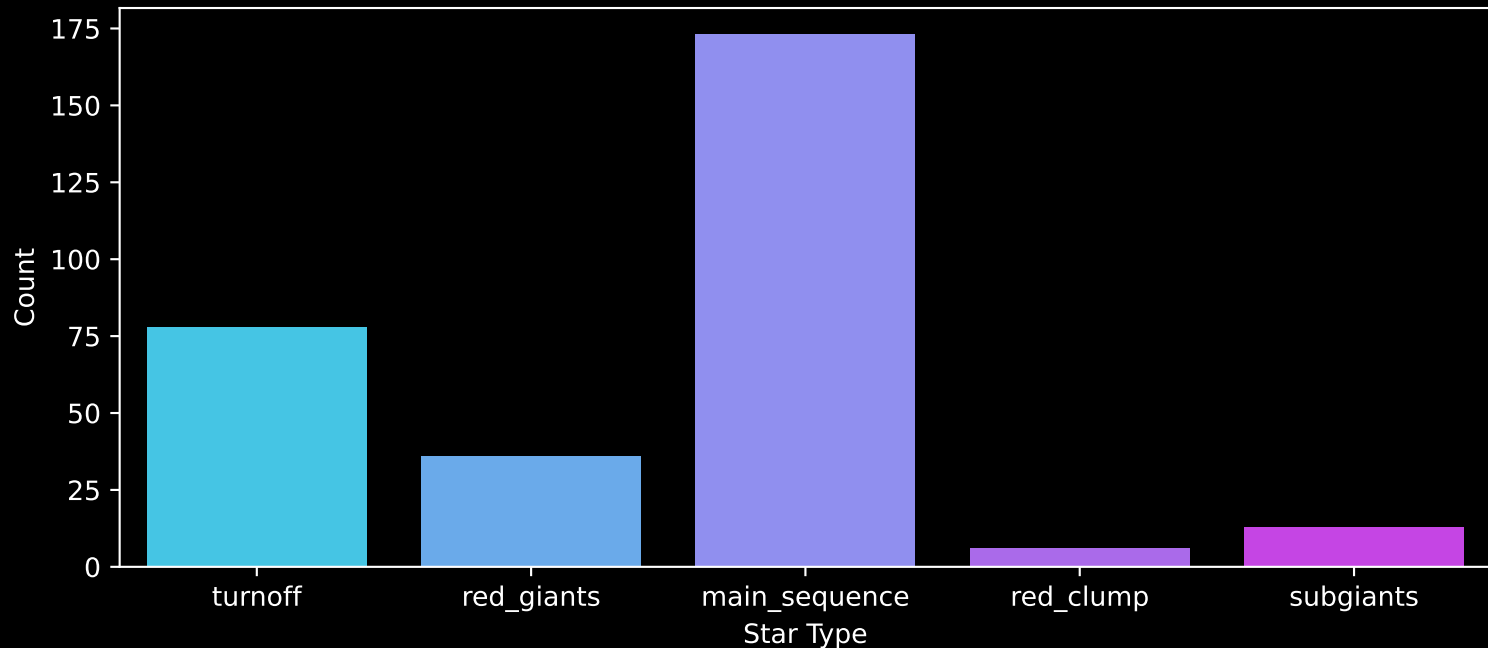
GALAH DR4 Field: [6965] Count plot of Star Type
