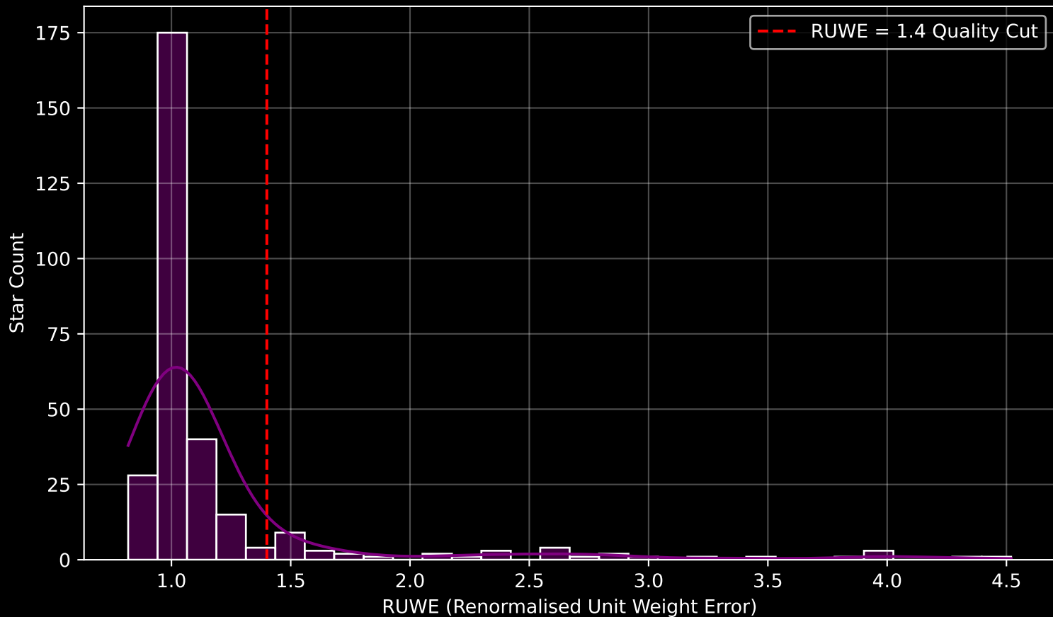
GALAH DR4 Field [6965] RUWE Distribution (n= 299)
