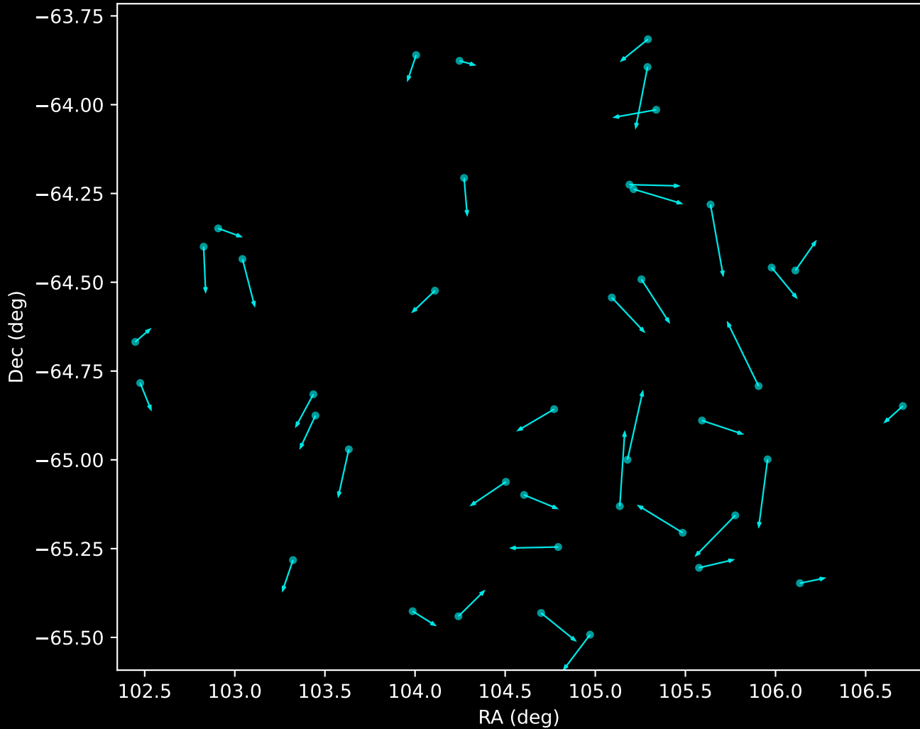
GALAH DR4 Noise Stream Proper Motion Vectors (n=41)
