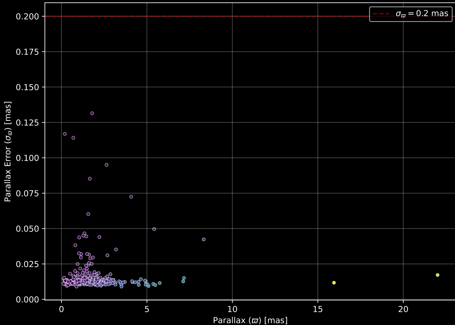
GALAH DR4 Field: [6965] Parallax Quality (n= 306)
